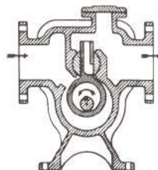
Fig. 9 Cam and Piston Pump
