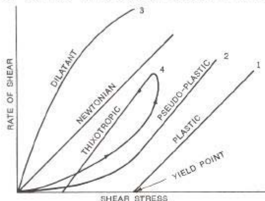
Fig. 14. Flow curves illustrating shear characteristics of various types of materials.
